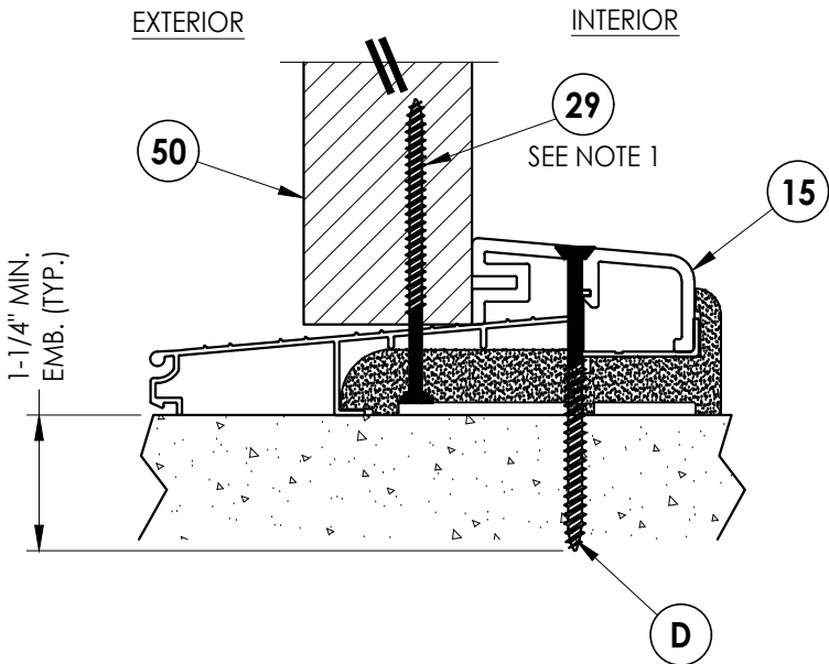
5 9 VERTICAL CROSS SECTION Outswing Threshold
