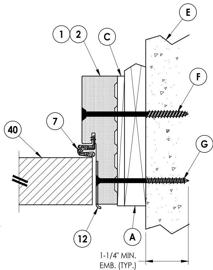
2 HORIZONTAL CROSS SECTION 7 Shown w/ 1X Buck Outswing shown (Inswing similar)
