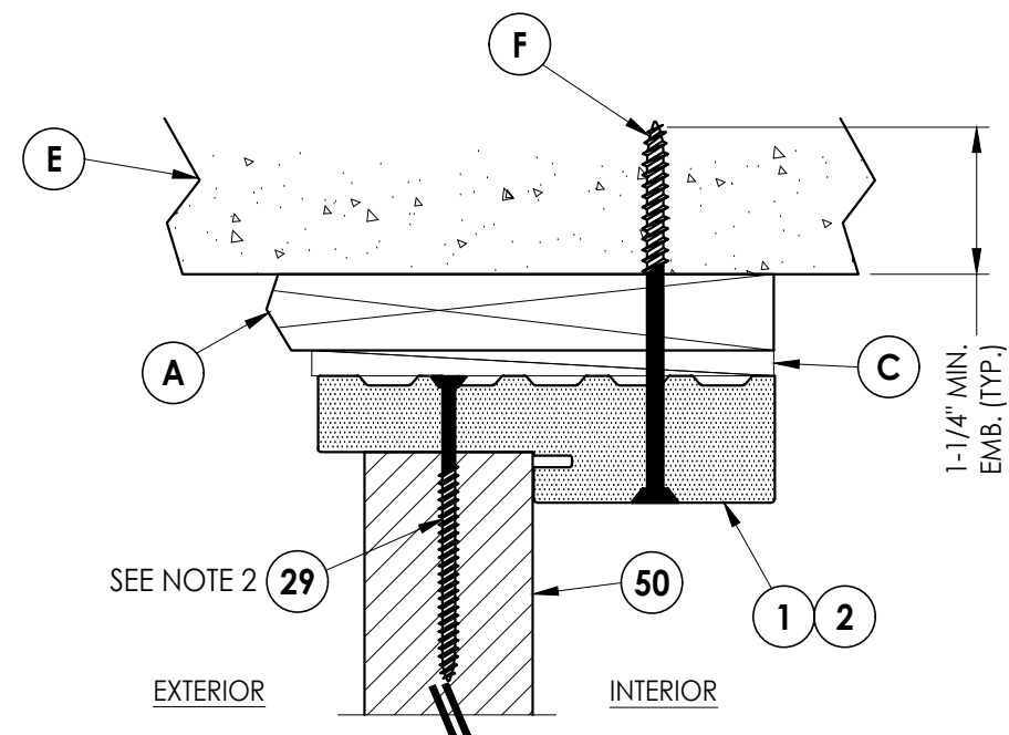
5 VERTICAL CROSS SECTION 7 Shown w/ 1X Buck Outswing shown (Inswing similar)
