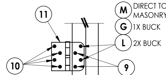
HINGE DETAIL
