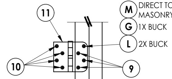
HINGE DETAIL
