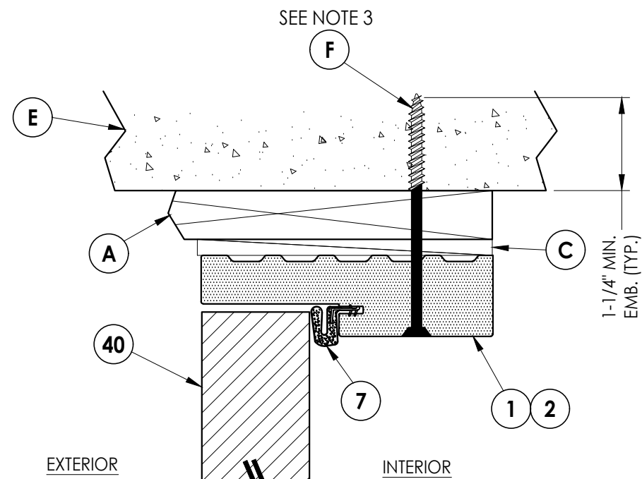
4 VERTICAL CROSS SECTION 7 Shown w/ 1X Buck Outswing shown (Inswing similar)
